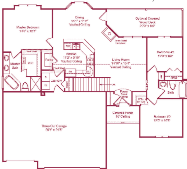
Main Level 1,300 sq. ft.
